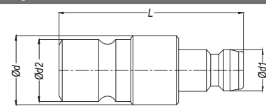
Adapting Plugs
